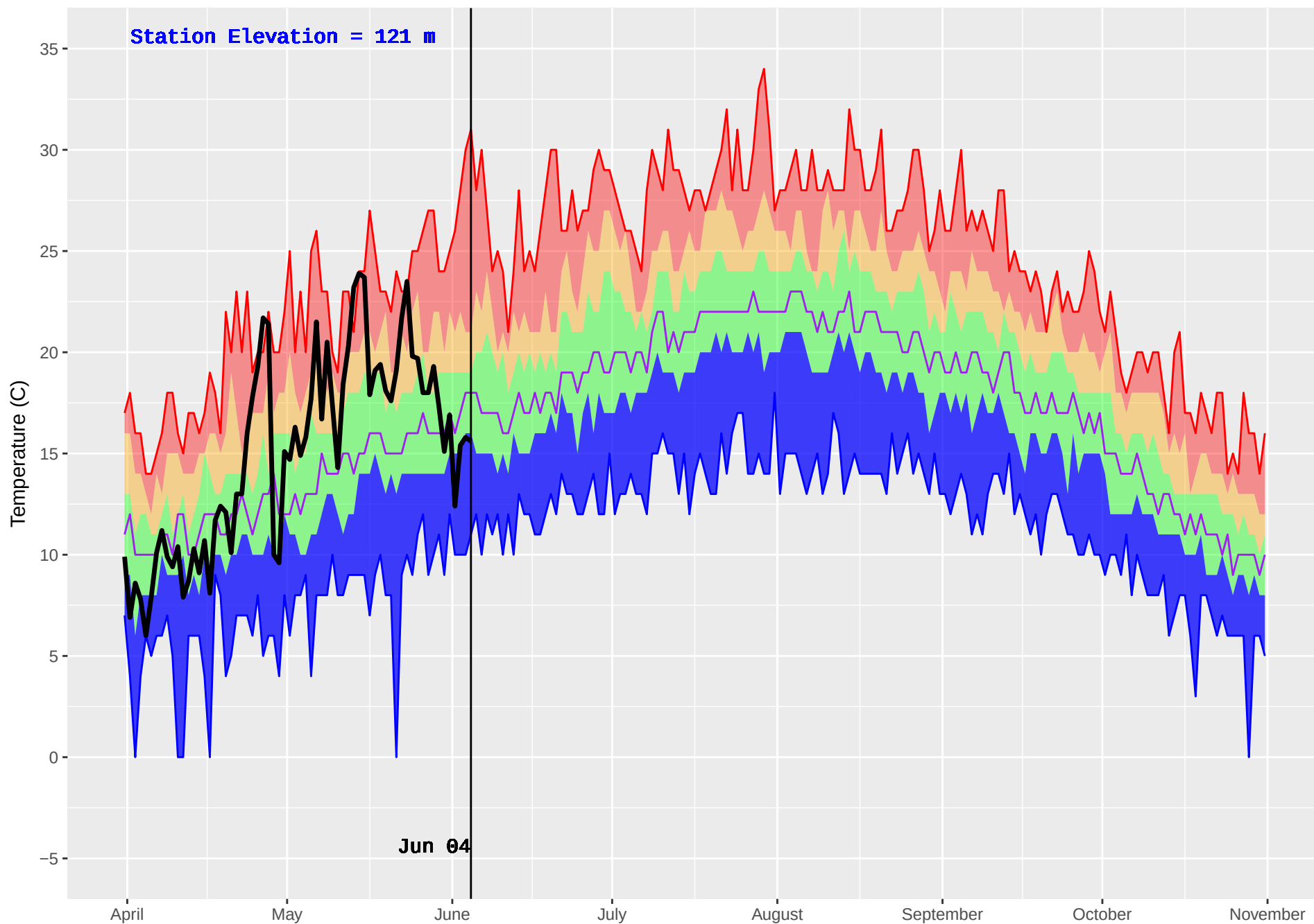
BOWSER (56) : Historical (1985–2016) and Current (2018) Noon Temperature
