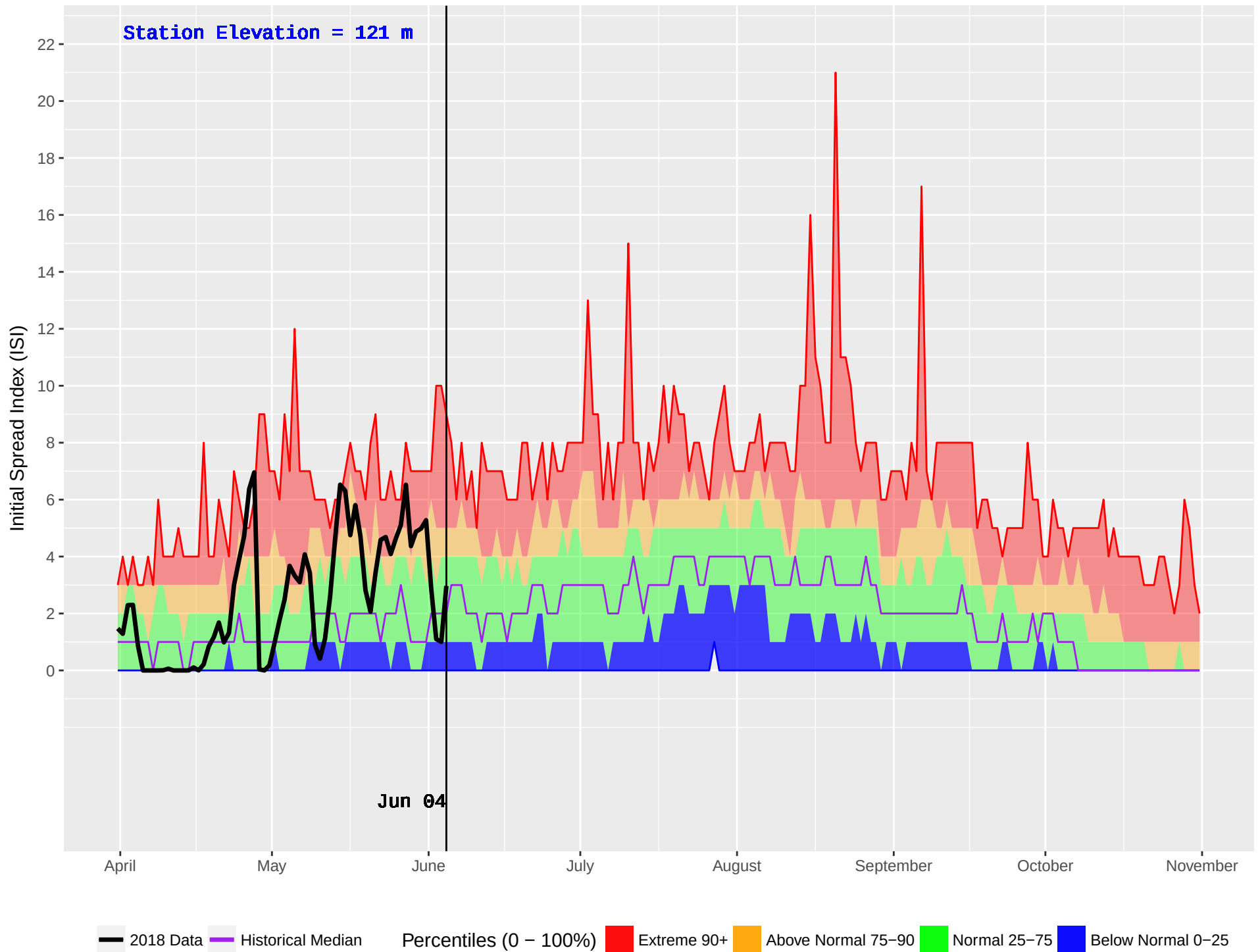
BOWSER (56) : Historical (1985–2016) and Current (2018) Noon Initial Spread Index (ISI)
