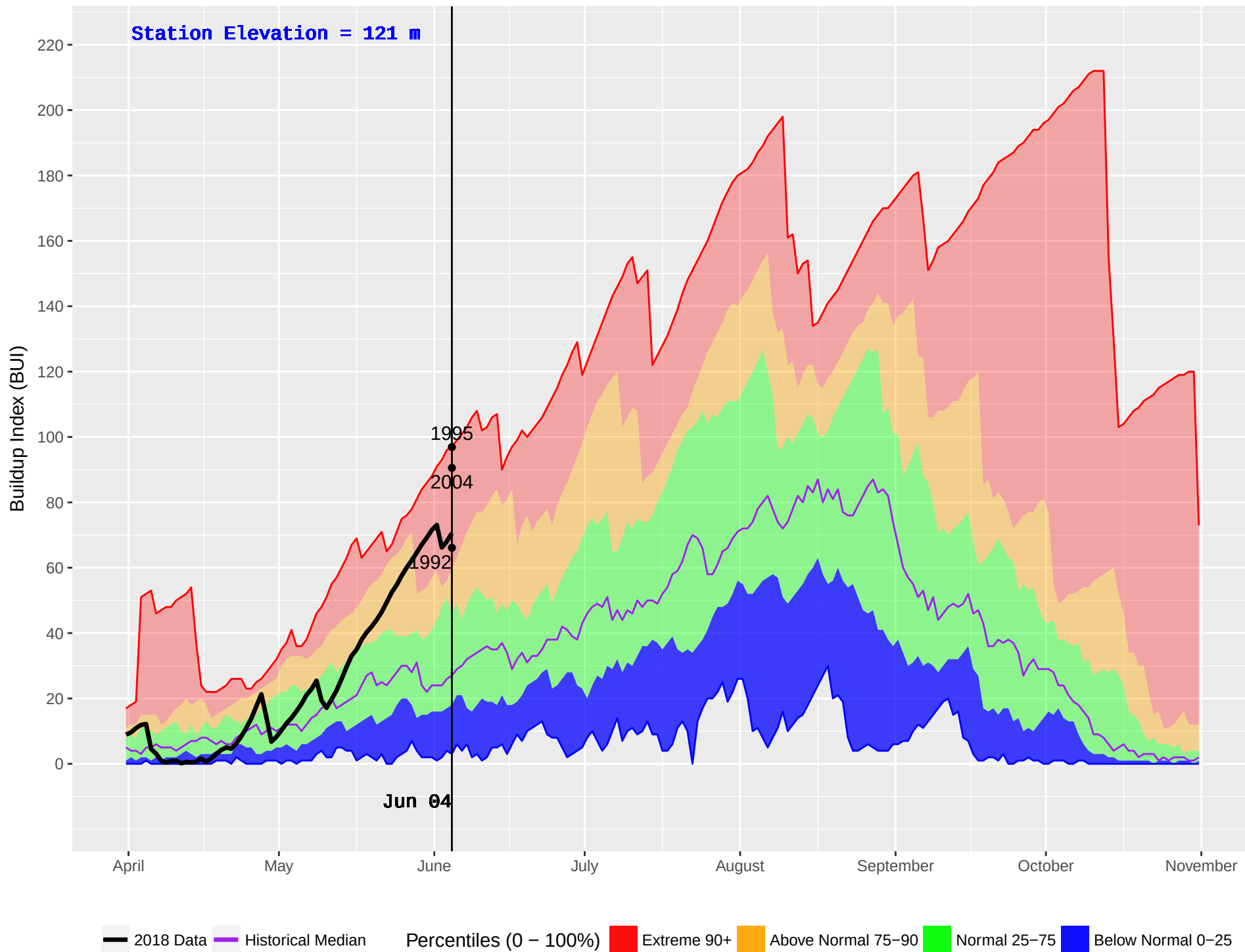
BOWSER (56) : Historical (1985–2016) and Current (2018) Noon Buildup Index (BUI)
